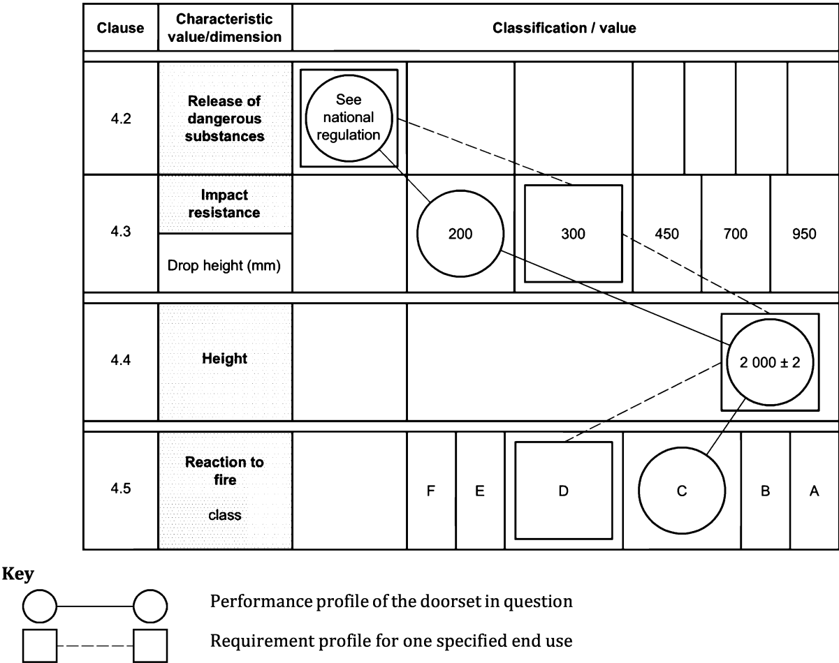
Figure C.1 — Example for performance and requirement profile of an internal pedestrian doorset
